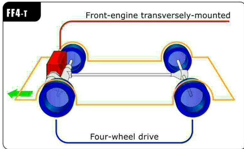
Alternate four-wheel drive
